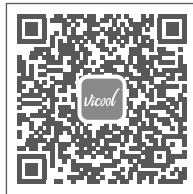
iOS Version
